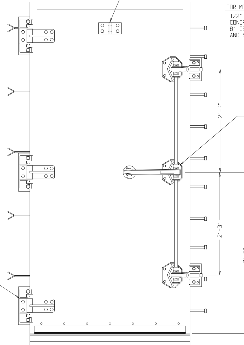
FRONT ELEVATION LEFT HAND SWING SHOWN - RIGHT HAND SWING OPPOSITE
