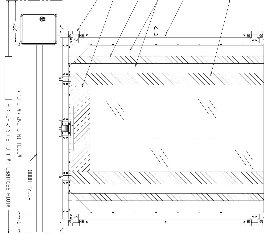
FRONT ELEVATION
