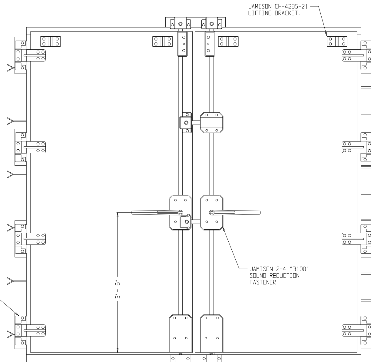
FRONT ELEVATION
